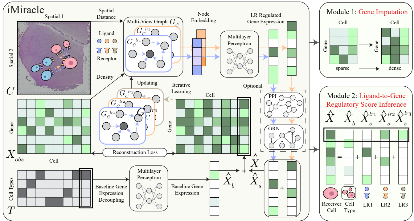
Figure 1: Overview of iMiracle. iMiracle initiates with a sparse cell-by-gene matrix X_{obs} \in \mathbb{R}^{n \times m} ( n cells and m genes), spatial coordinates C \in \mathbb{R}^{n \times 2} , and cell type information T \in \mathbb{R}^{n \times t} ( t cell types). It constructs multi-view cell-cell communication networks G_C to model various ligand-receptor interactions. Node embeddings for each cell are generated per view through a graph neural network. A multilayer perceptron then decodes gene expression \hat{X}_s influenced by these LR interactions, integrating knowledge from an established gene regulatory network. iMiracle isolates the baseline gene expression matrix \hat{X}_b solely determined by cell types. The final imputed gene expression matrix \hat{X} merges the baseline matrix with expressions from ligand-receptor interactions. Through iterative learning, \hat{X} is used to progressively refine the multi-view graph, enhancing both imputation precision and the inference of ligand-to-gene regulatory scores.
